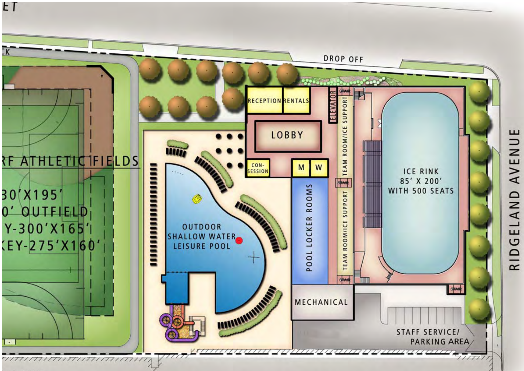
FIRST FLOOR
